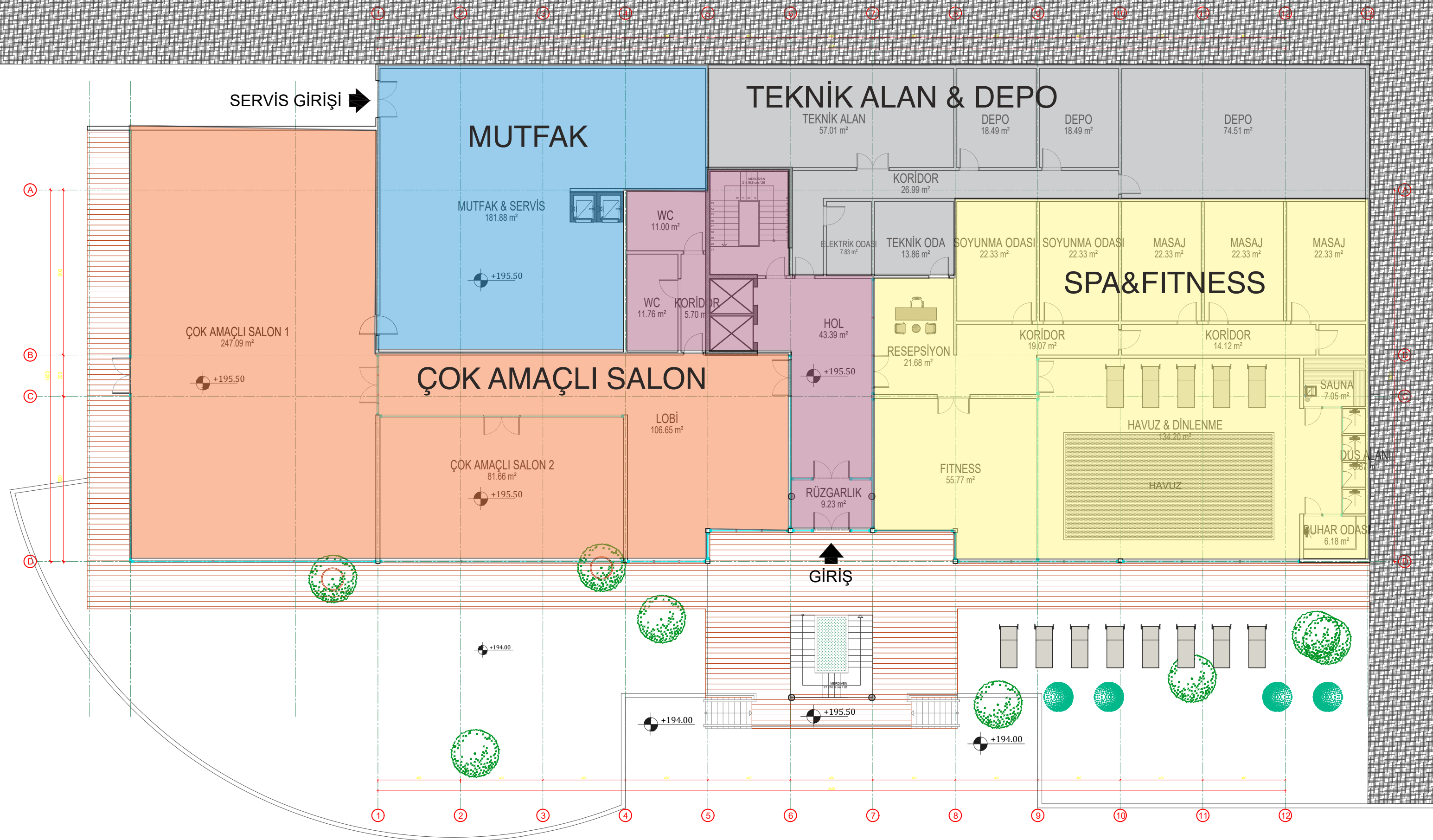
HOTEL - BODRUM KAT PLANI
